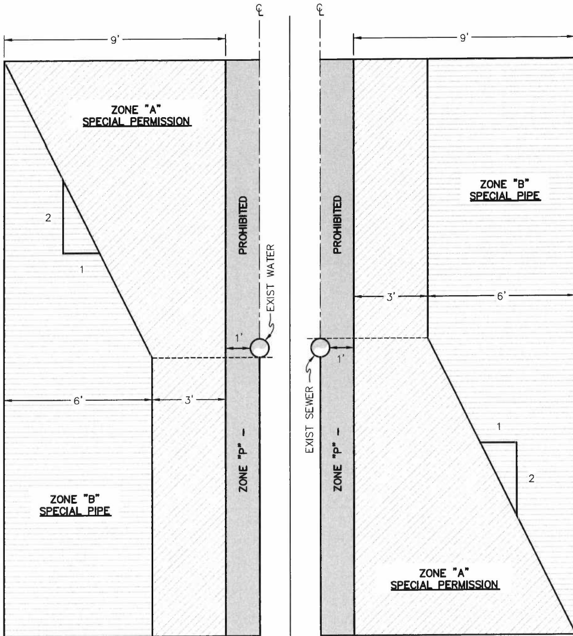
FIGURE 1 – PARALLEL CONSTRUCTION SECTIONAL VIEW
