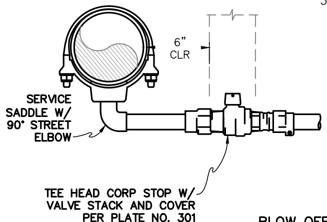
BLOW OFF CONNECTION AT LOW POINT ON MAIN
